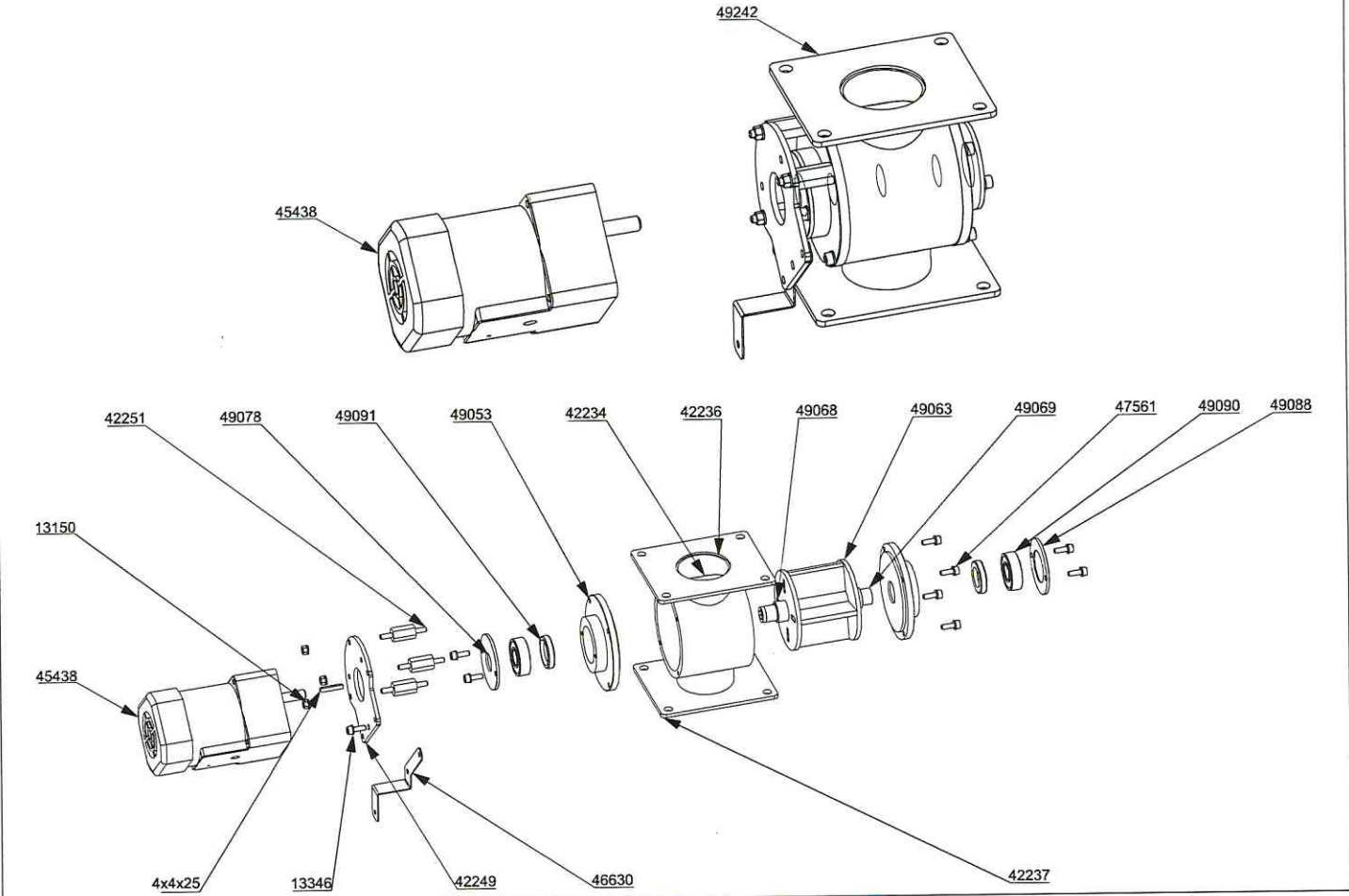
EXPLODED VIEW OF THE BOILER BIOTEC PLUS 25 - side - PELLET - rotary valve of pellet delivery
